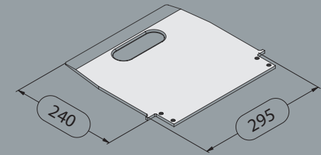
Standard toe plate 295 x 240 mm
