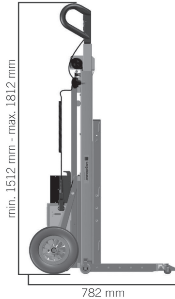
(Fork Plate Dimension)
